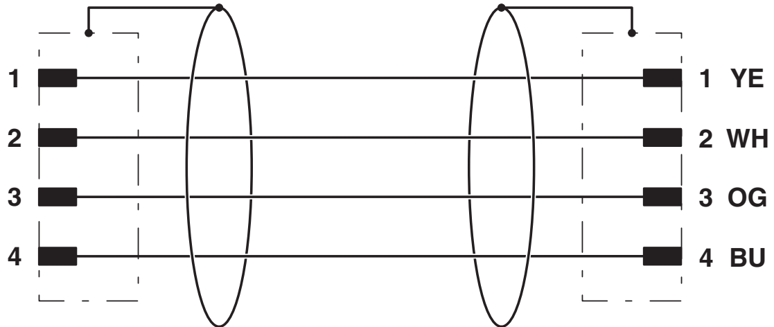
Contact assignment of the M12 plugs
