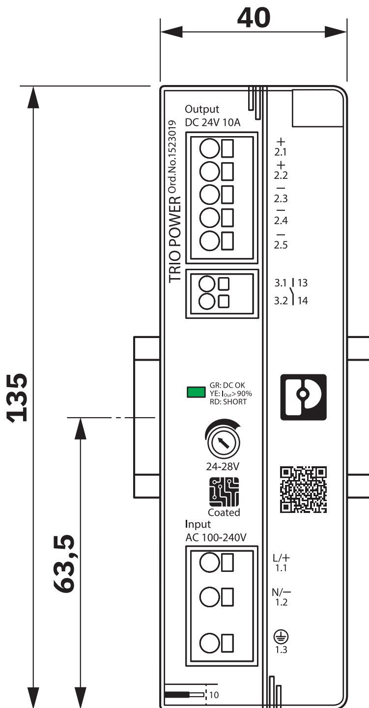
Dimensional drawing
