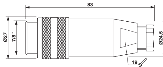
Dimensional drawing
