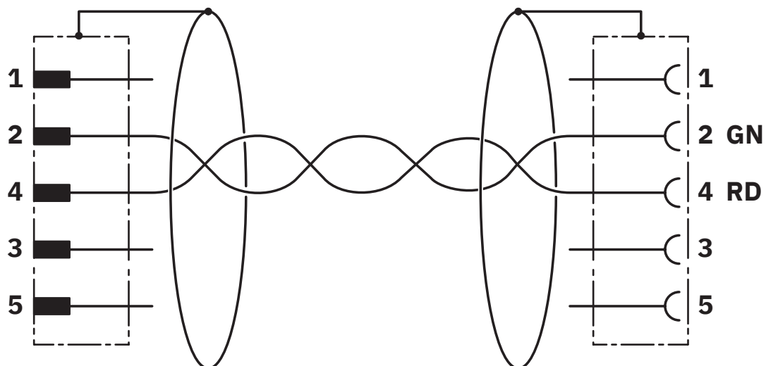
Circuit diagram
