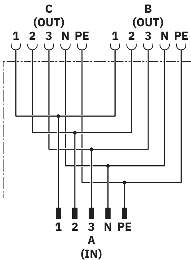
Circuit diagram
