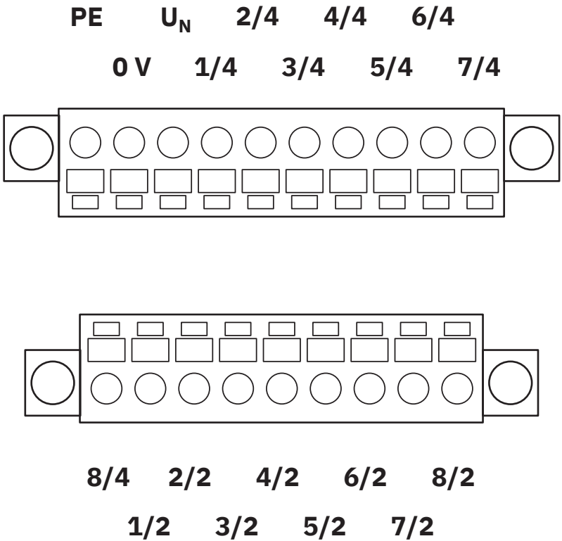
Schematic drawing of terminal assignment of PCB terminal block
