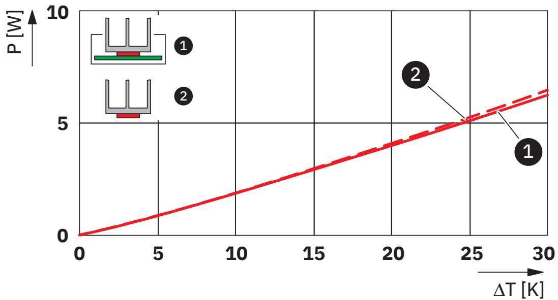
Power dissipation diagram for 0 K ... 30 K
