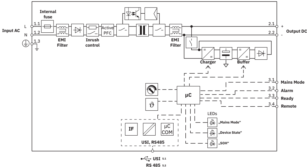
Block diagram
