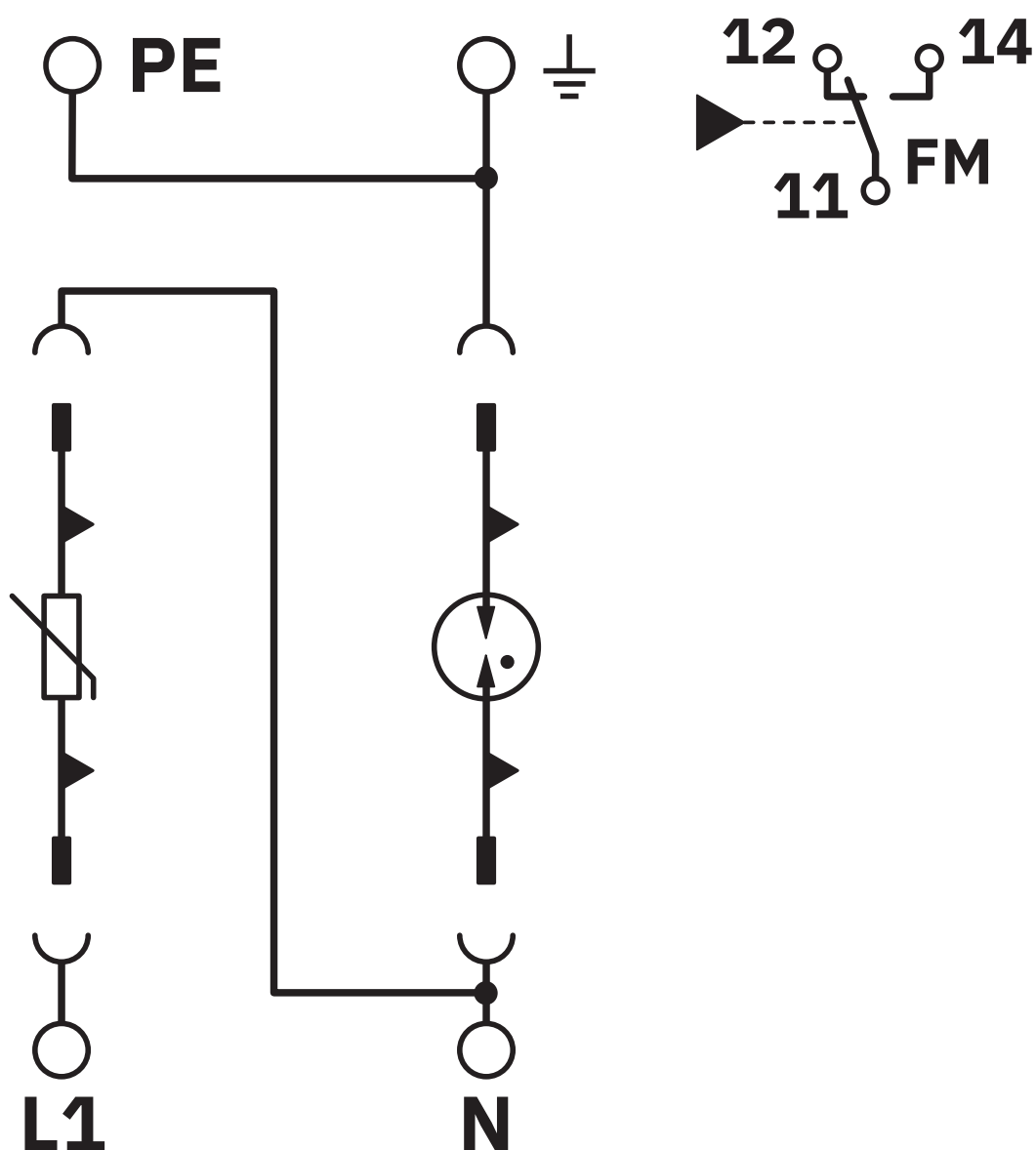
Circuit diagram
