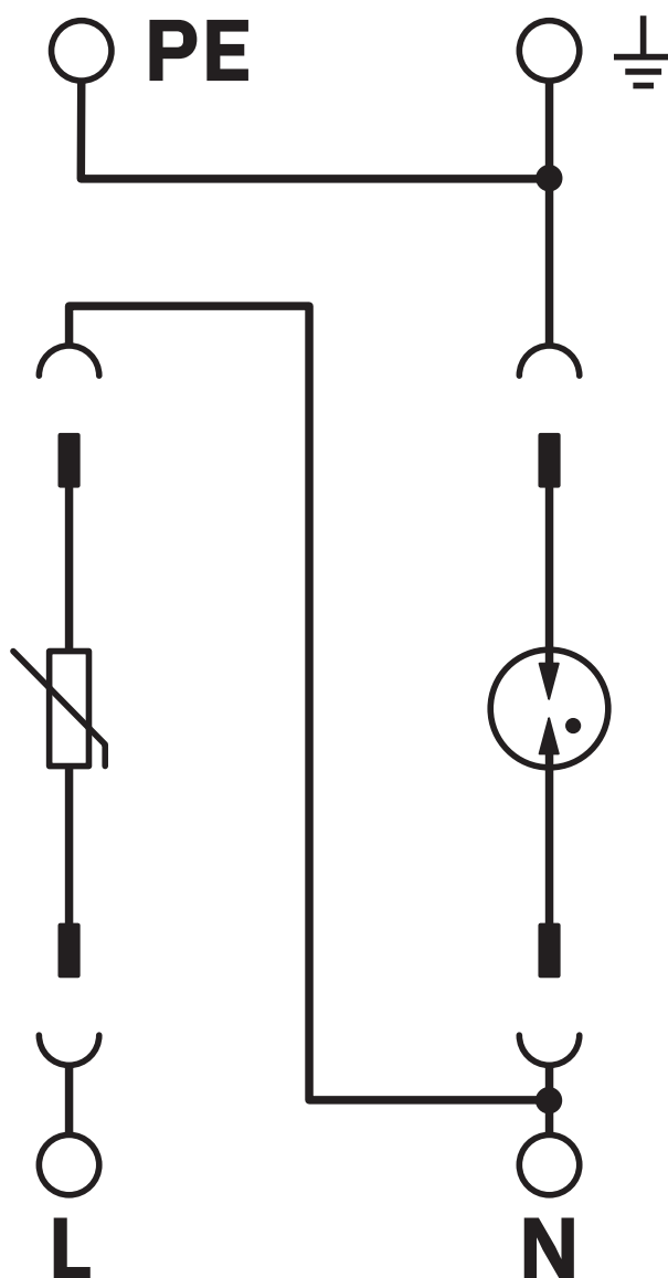
Circuit diagram
