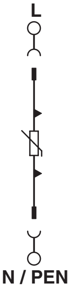
Circuit diagram
