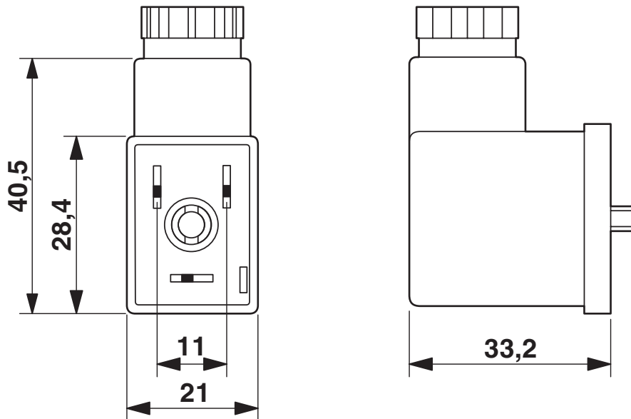
Dimensional drawing
