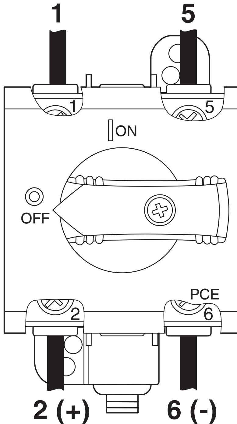
Connection diagram
