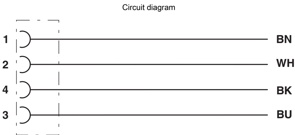
Contact assignment of the M12 plug
