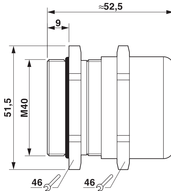
Dimensional drawing
