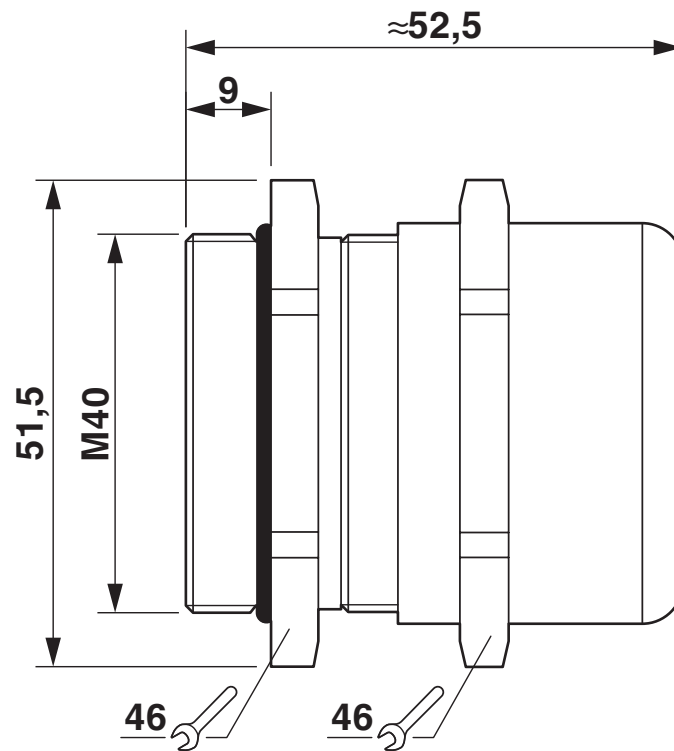
Dimensional drawing
