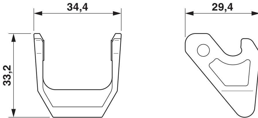
Dimensional drawing
