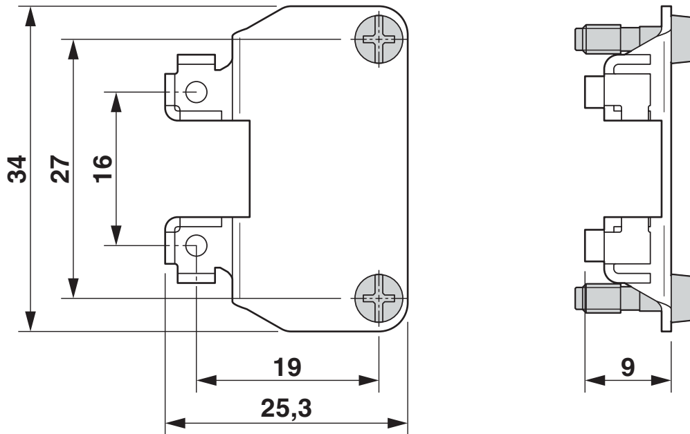
Dimensional drawing
