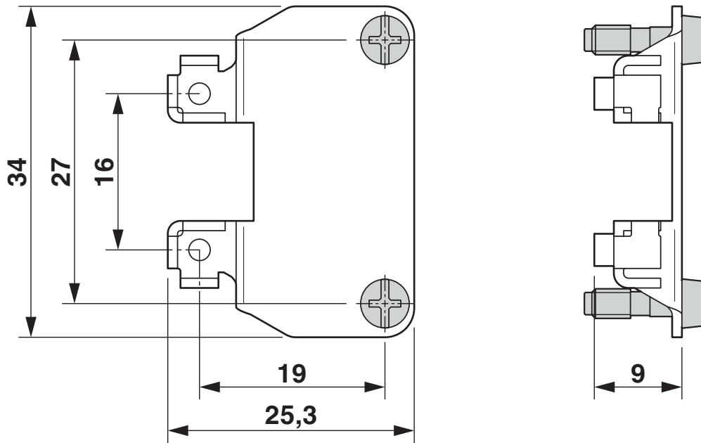
Dimensional drawing
