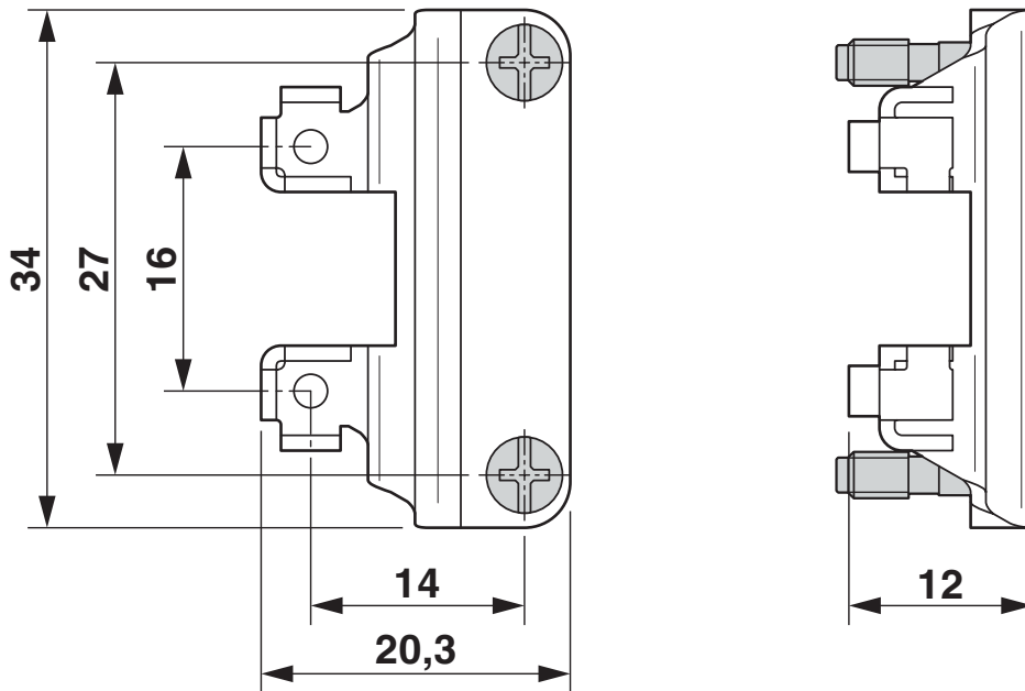
Dimensional drawing
