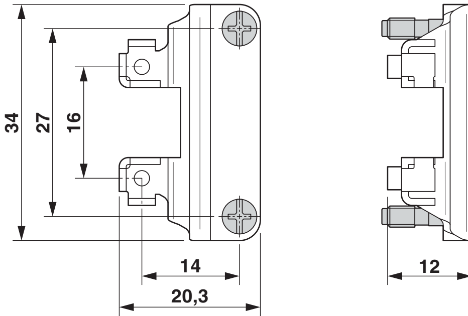
Dimensional drawing
