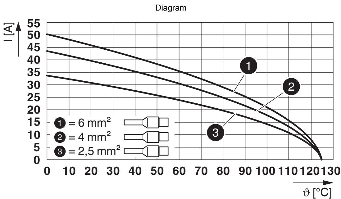
Derating diagram for flexible conductors with ferrule
