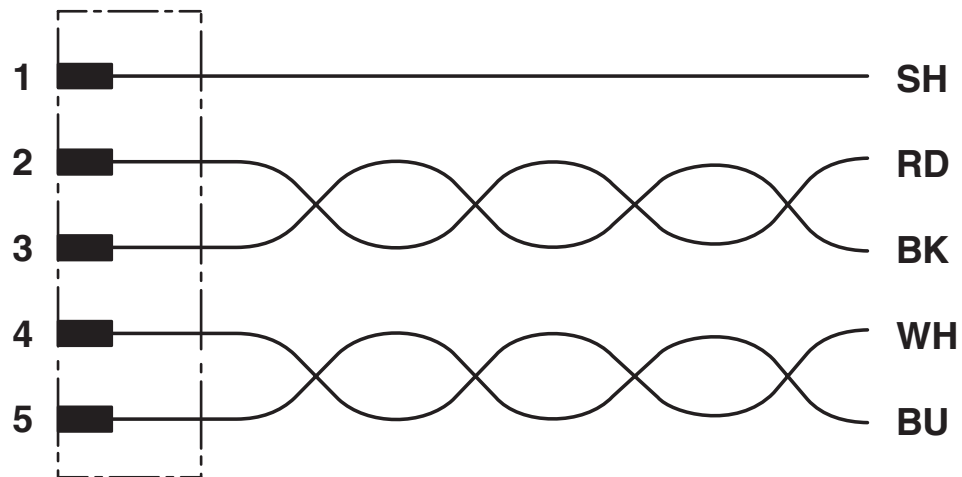
Contact assignment of the M12 plug
