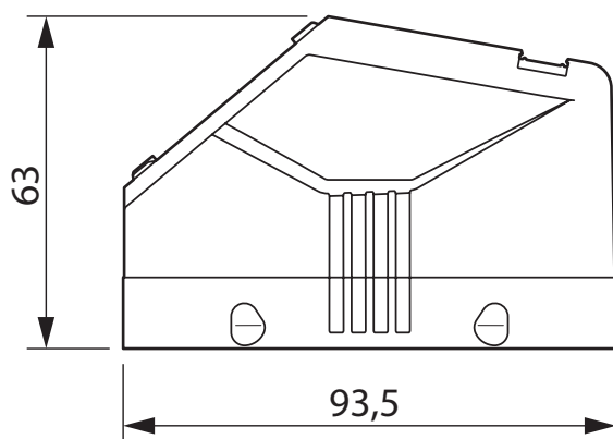
Dimensional drawing
