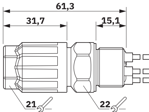
Dimensional drawing
