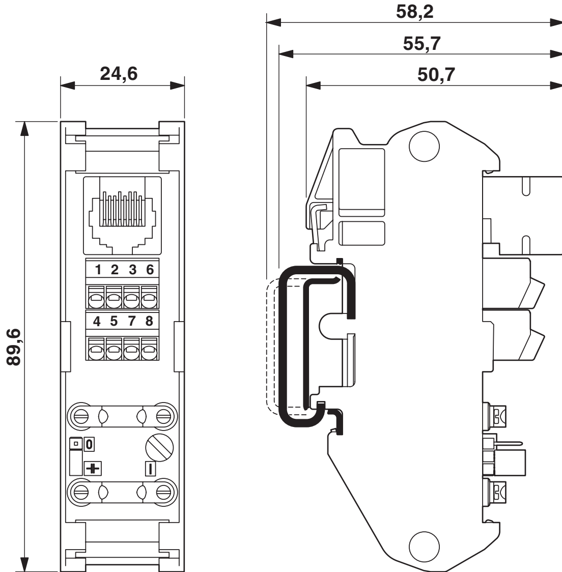
Dimensional drawing
