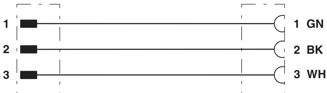
Circuit diagram
