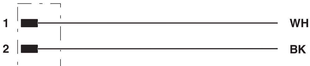
Contact assignment of 7/8" plug
