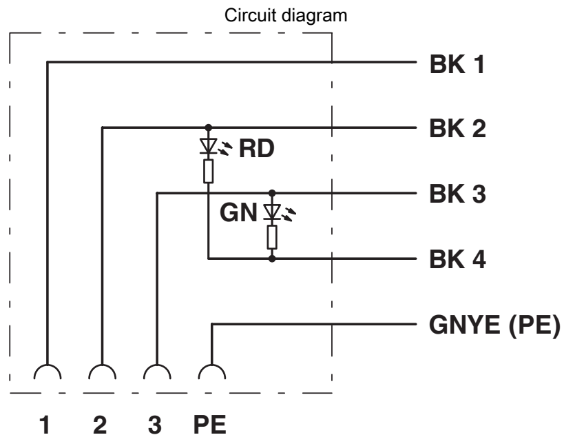
Valve plug connector pin assignment, type AD
