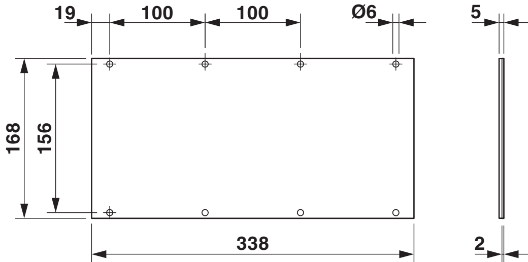
Dimensional drawing
