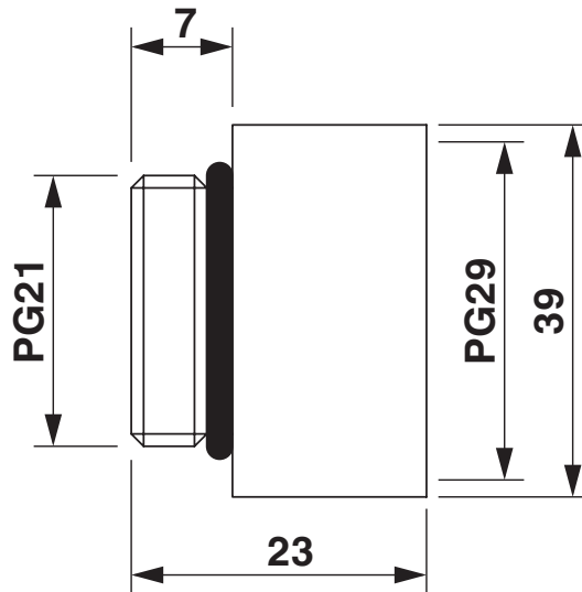
Dimensional drawing
