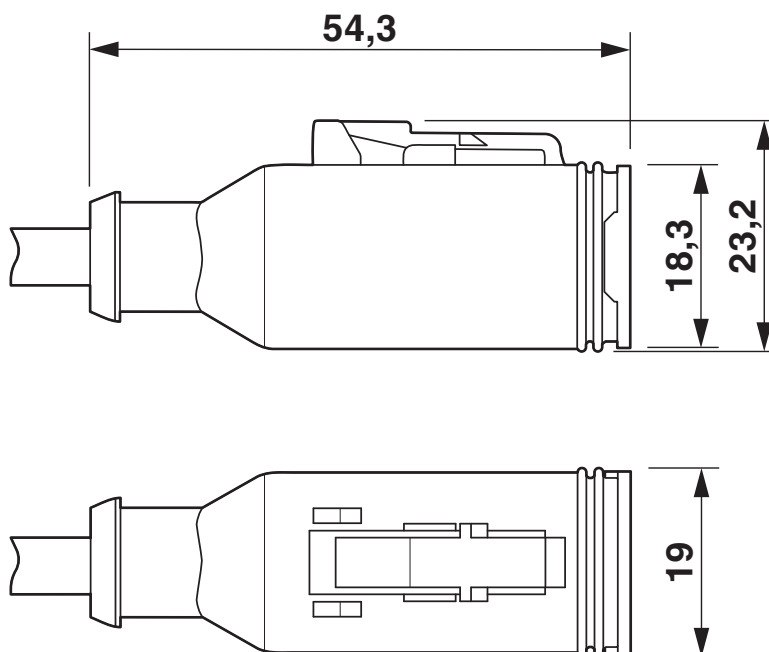
Dimensional drawing
