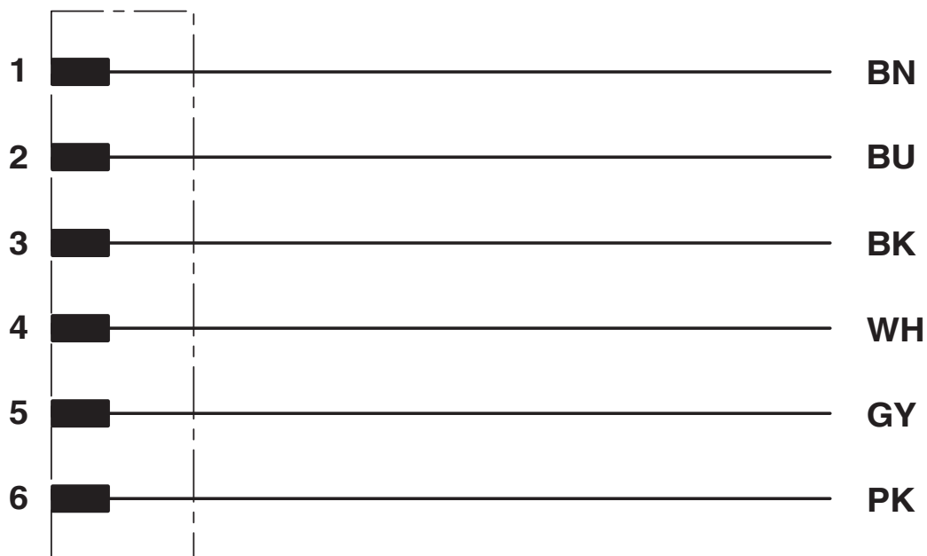
Contact assignment of the DEUTSCH DT04-6P
