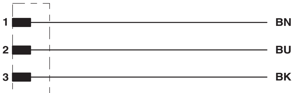
Contact assignment of the DEUTSCH DT04-3P
