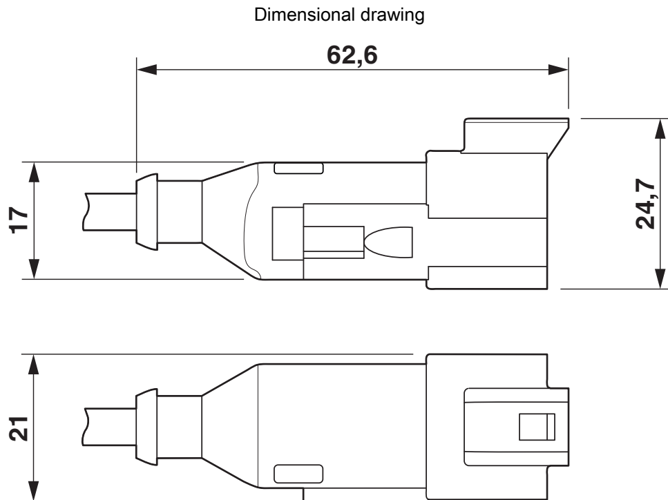
DEUTSCH DT04-3P, top view and side view
