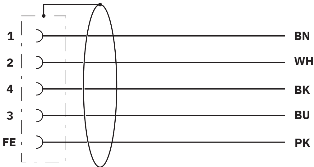
Contact assignment of the M12 socket
