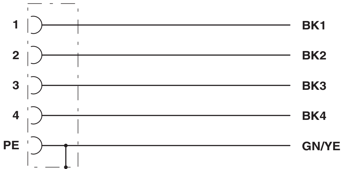
Contact assignment of the M12 socket
