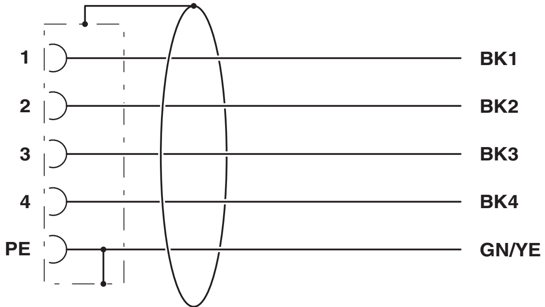
Contact assignment of the M12 socket
