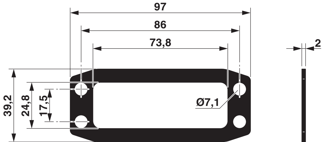
Dimensional drawing
