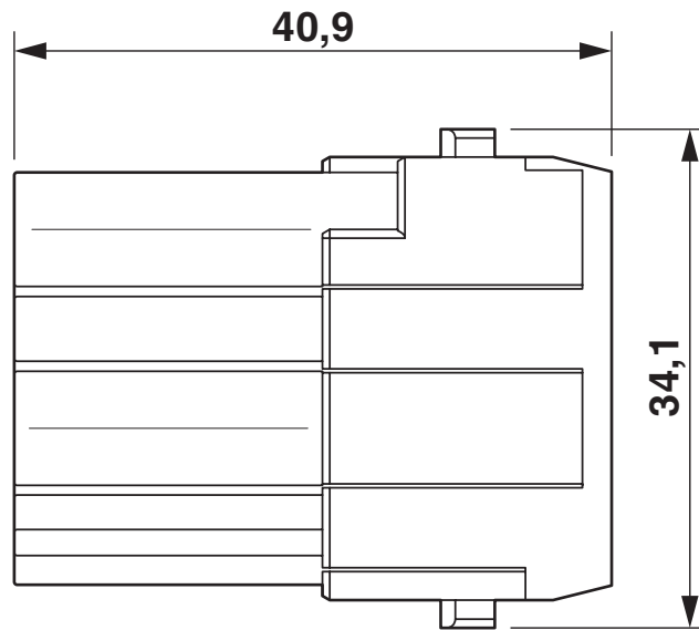
Dimensional drawing
