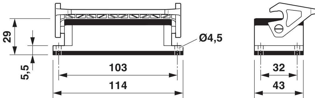
Dimensional drawing
