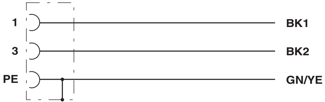
Contact assignment of the M12 socket
