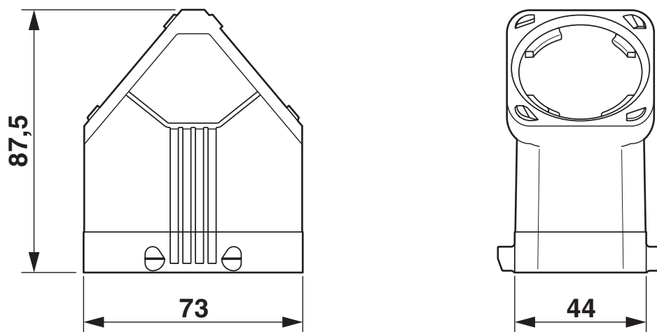
Dimensional drawing
