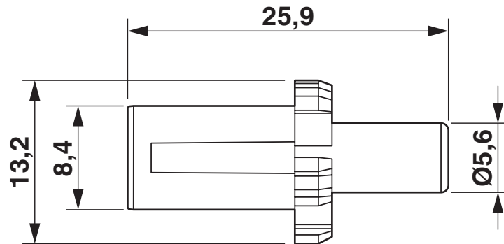
Dimensional drawing
