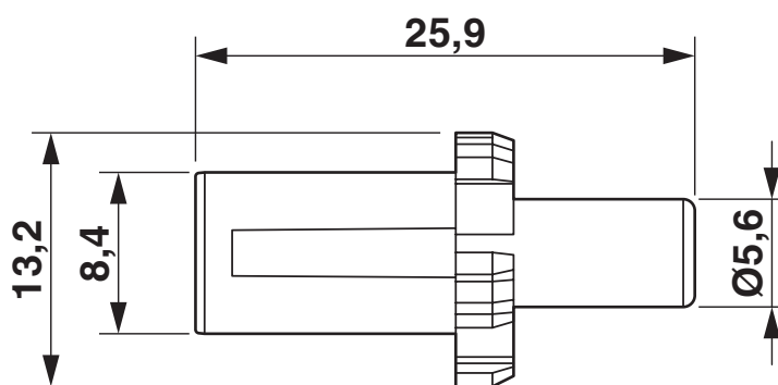
Dimensional drawing
