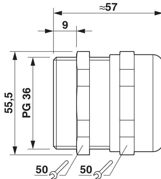
Dimensional drawing
