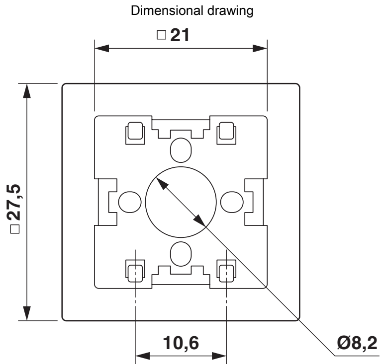
Dimensional drawing
