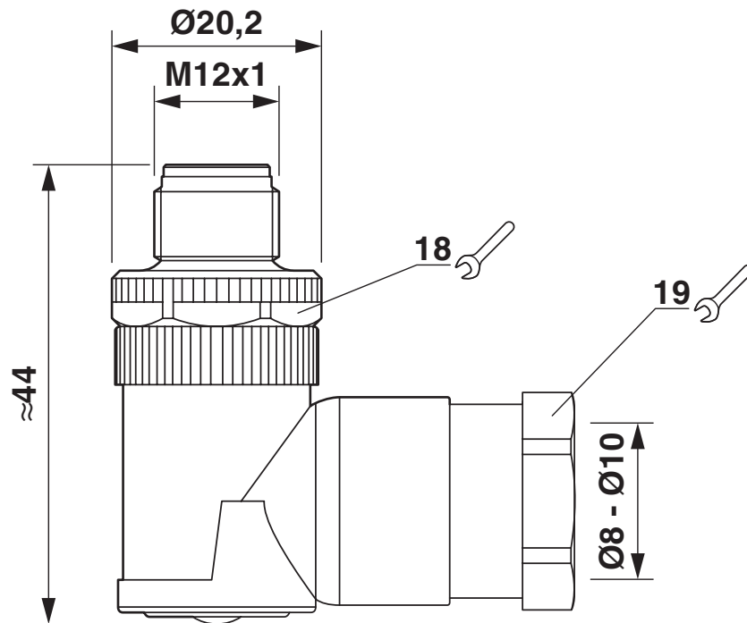
Dimensional drawing
