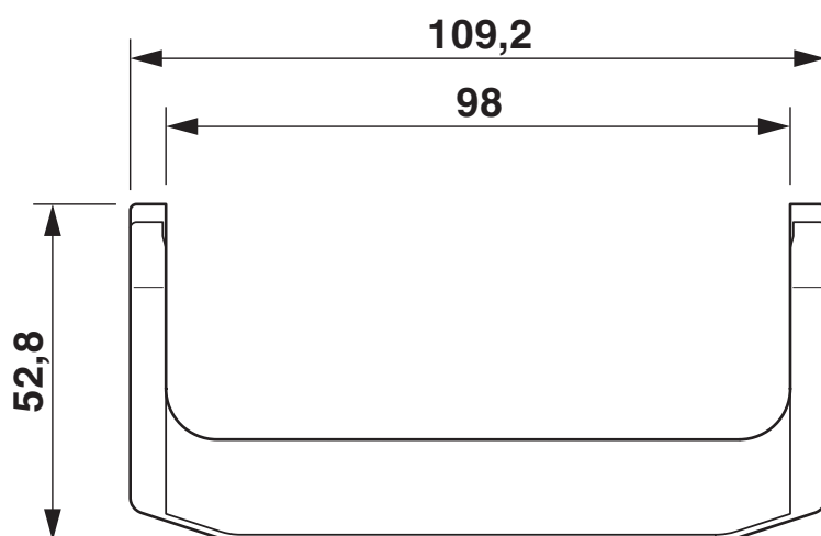
Dimensional drawing
