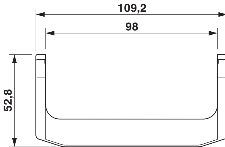
Dimensional drawing
