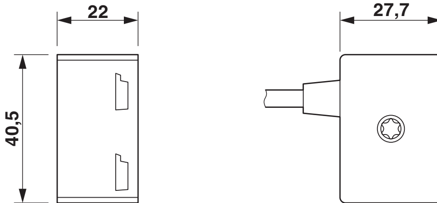
Dimensional drawing
