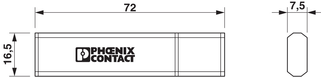
Dimensional drawing
