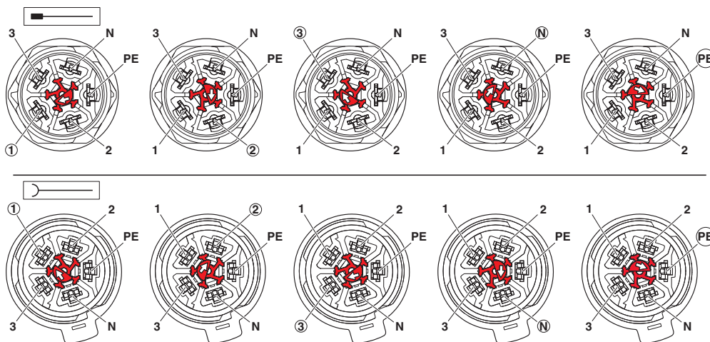
Functional drawing
