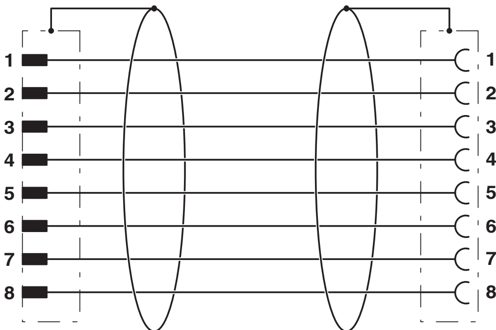
Contact assignment of M8 plugs/sockets
