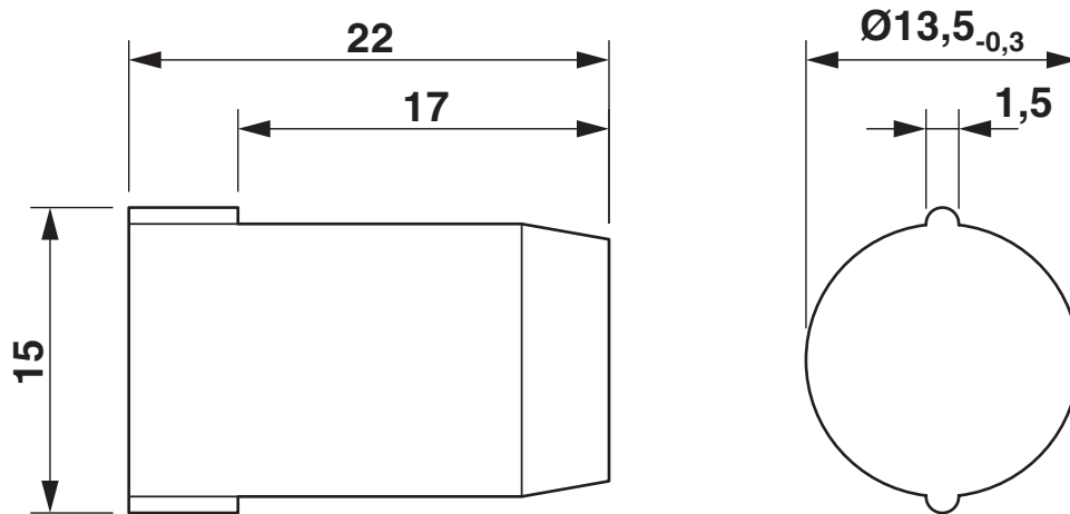
Dimensional drawing
