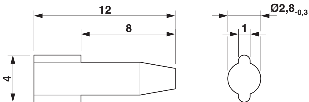
Dimensional drawing
